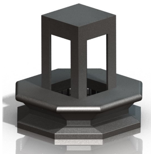
4 Section Premier Carousel #PR2402 & 2403 Shown with inserts, security panels and security panel top filler. Dimensions: 67.1x54x58T
