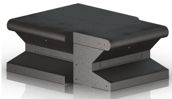
3 Premier Slot Base Back-to-Back # PR1203 Shown with Mouse Hole Kit Dimensions: 46Dx36Wx18T
